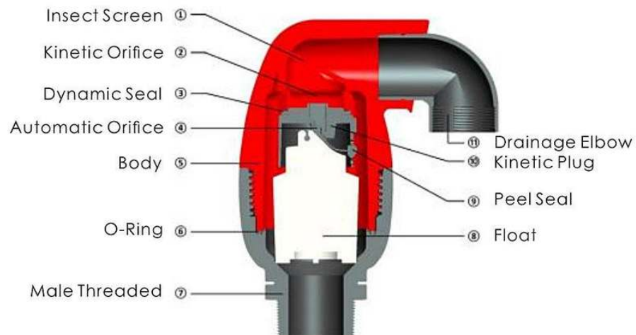
Air Relief and Intake (Pipeline Filling, Draining and Vacuum Conditions)
