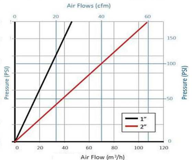
Air Release (Pressurized Operation)
