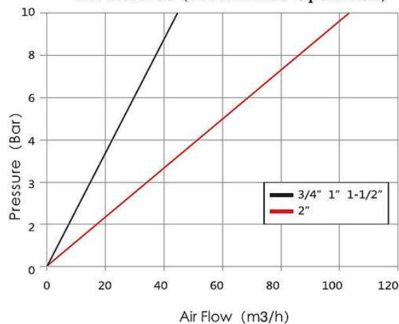
Air Release (Pressurized Operation)
